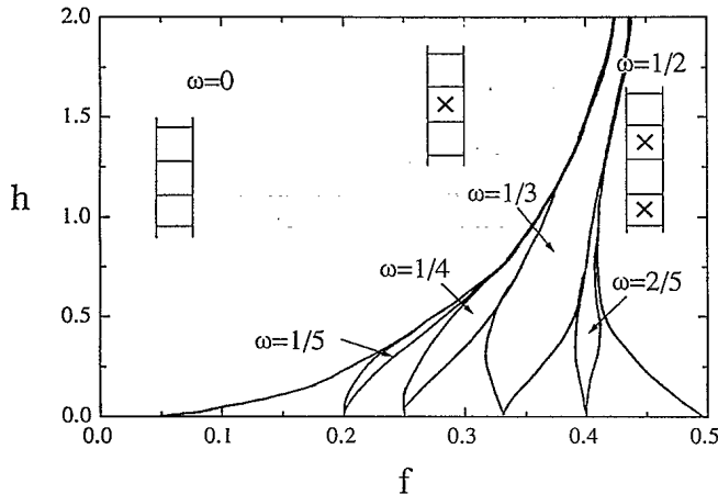
FIG. 2. The phase diagram of the JJ ladder obtained using the method of effective potentials. Each phase is defined by the value of \omega and, for clarity, only a few of the transition lines are represented. The sketches of the ladders show the vortex configurations of the simplest commensurate states.
