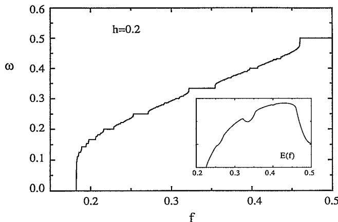
FIG. 3. \omega(f) for the ground-state configurations when h = 0.2 . This function is a devil's staircase: a continuous function with an step for each commensurate value of \omega . The inset shows the continuity of the ground-state energy as a function of the frustration.
