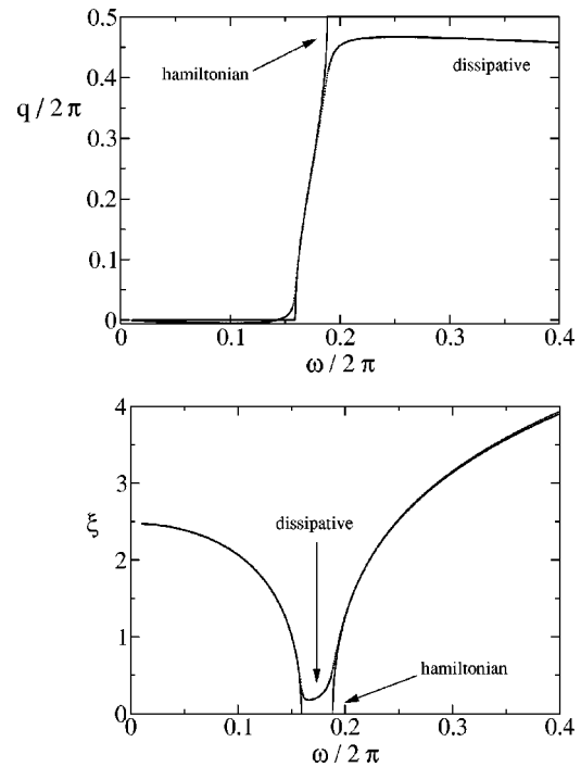
FIG. 3. Tail analysis for a rotobreather in a Josephson junction ladder. Wave vector q and inverse decay length \xi as functions of \omega for the ladder parameters ( J_y = 0.5, J_x = 0.1, \epsilon_x = \epsilon_y = 0.01 ). For the latter, and outside the “phonon band,” the Hamiltonian and dissipative solutions almost overlap in spite of the differences between both cases shown in the q variable.
