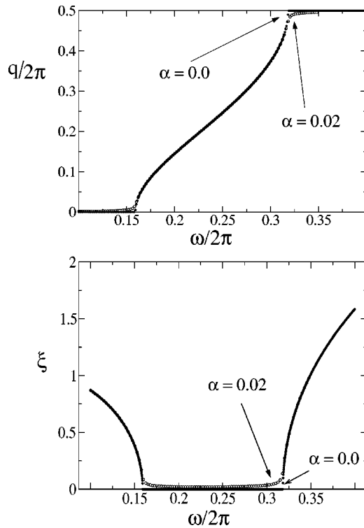
FIG. 2. Tail analysis of dissipative DB's in the Frenkel-Kontorova model. Wave vector q and inverse of the decay length \xi as functions of \omega for two different values of the damping, \alpha = 0.02 (open circles) and the Hamiltonian case \alpha = 0.0 (filled ones). The coupling parameter C is in both cases equal to 0.75.
