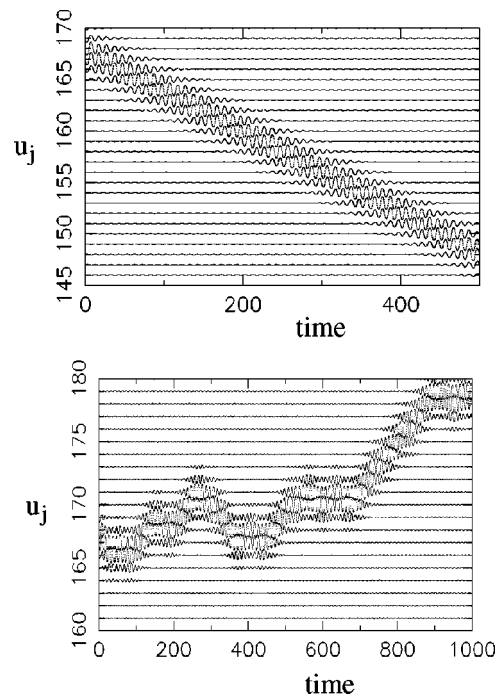
FIG. 10. The upper figure shows a MB with regular motion at C=0.75 . Below, a MB with diffusive motion at C=0.65 .
