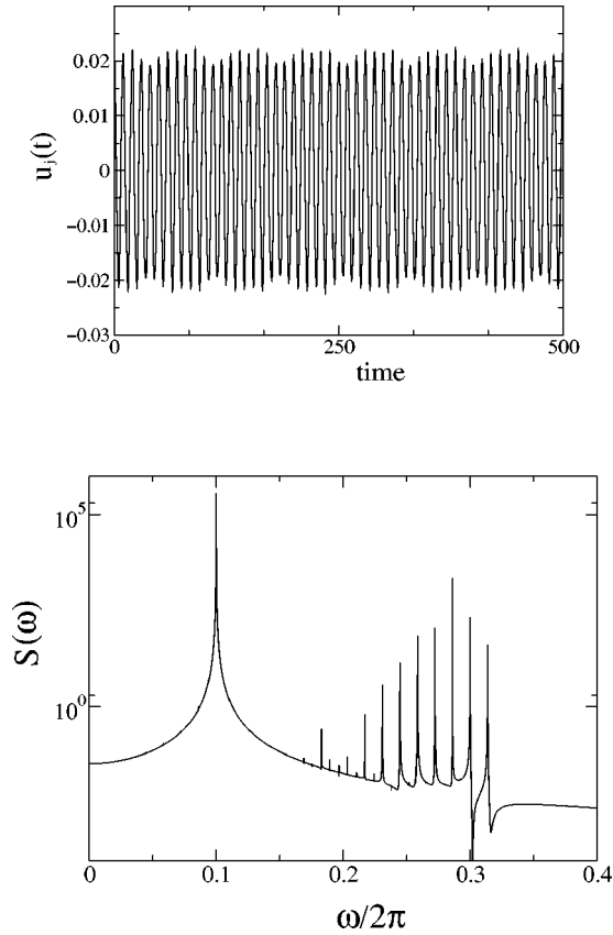
FIG. 12. Time evolution for the tail of quasiperiodic breather at C=0.817 (upper figure) and the corresponding power spectrum (down figure) whose peaks are given by linear combinations of two frequencies \omega_b and \omega_{\text{new}} .
