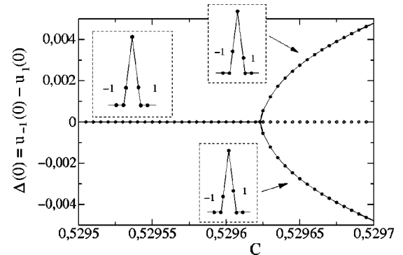
FIG. 5. Profiles of the breather around the area of the pitchfork bifurcation.
