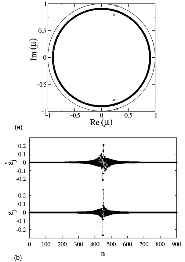
FIG. 6. Floquet spectrum for the Hopf bifurcation at C = 0.871 . An eigenvalue and its complex conjugate cross the unit circle at a nonzero angle in the complex plane. The figure at the bottom shows the corresponding eigenvector.
