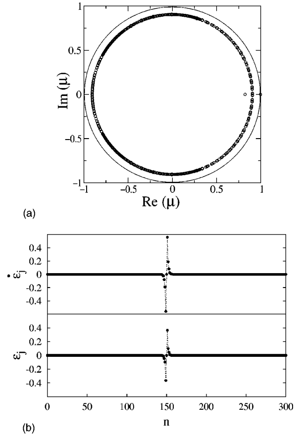
FIG. 4. Floquet spectrum for the one-site breather near C = 0.5296 and closely after the first pitchfork bifurcation. All eigenvalues are in a circle of radius \exp(-\alpha t_b/2) except two, one of which crosses the unit circle by +1 . The lower figure shows the profile of the eigenvector corresponding to this unstable eigenvalue (both velocity and position components, \epsilon_i , \dot{\epsilon}_i ). Note that it is antisymmetric and strongly localized.
