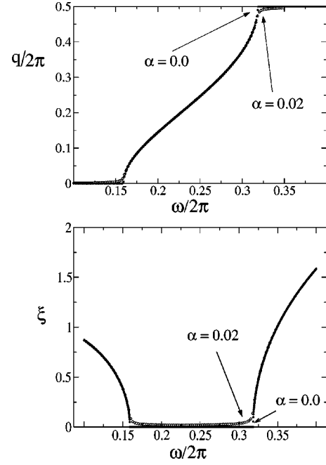
FIG. 1. Wave vector q and inverse of the decay length \xi as functions of \omega for two different values of the damping, \alpha=0.02 (open circles) and the Hamiltonian case \alpha=0.0 (filled ones). The coupling parameter C is in both cases equal to 0.75.
