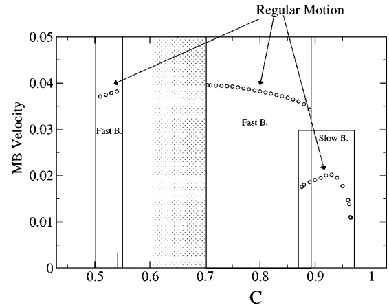
FIG. 9. Velocity of MB vs coupling parameter C . Dashed area shows the region in which MB have a diffusive motion. It is also showed different regions of “slow” and “fast” MB. See the text for details.
