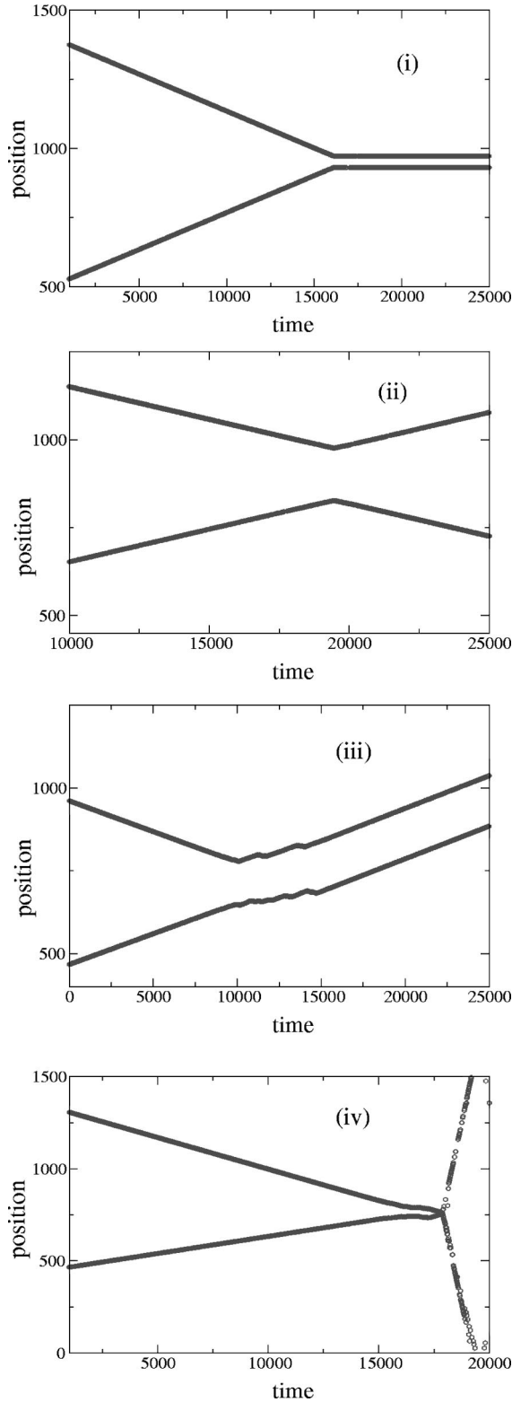
FIG. 15. Four scenarios of collisions between breathers. We represent the traces by plotting the position of the energy maximum. (i) Formation of a pinned ‘‘molecule’’ after a collision of two MB at C=0.75 and F_{ac}=0.011 ; (ii) ‘‘elastic’’ collision at C=0.89 and F_{ac}=0.02 ; (iii) Formation of mobile ‘‘molecule’’ C=0.89 and F_{ac}=0.02 ; (iv) Annihilation of a ‘‘slow’’ and a ‘‘fast’’ breather at C=0.89 and F_{ac}=0.02 . In this last case, the traces after the collision correspond to linear radiation (phonons).
