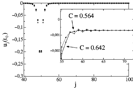
FIG. 3. Breather profiles (two-site breathers) at a given time for two different values of C (0.564 filled circles and 0.642 open ones, see also Fig. 2). The inset shows the right-hand-side tails, where we can observe the existence of a phonon in the second case, corresponding to the entrance of the third harmonic of \omega_b in the phonon band. The points are connected as a guide to the eye.
