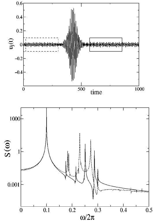
FIG. 13. Time evolution for a particle that is passed by a MB (upper). Below, power spectra corresponding to the tails before and after the passage of the breather. Note how the peaks are shifted by Doppler effect.
