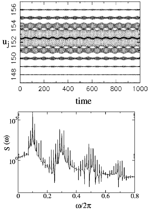
FIG. 7. Two-site quasiperiodic breather. Note that particles on both sides of the breather are out of phase. The figure below shows the power spectrum of one of the central particles. The peaks are linear combinations of the two relevant frequencies, \omega_b and \omega_{new} . Note that only odd harmonics of \omega_b appear.
