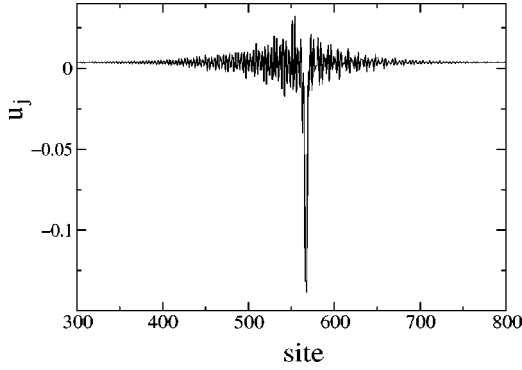
FIG. 11. Instantaneous profile of a MB at C=0.75 and F_{ac}=0.045 . Note the clear asymmetry of the phonon tails in front of and behind the breather.
