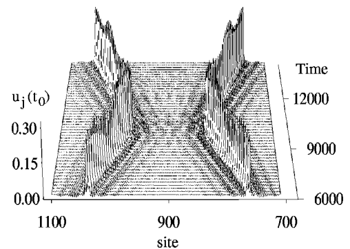
FIG. 14. An elastic collision between two slowly moving breathers. It is possible to appreciate how the breathers “see” each other through their phonon tails. This collision was obtained at C=0.89 .
