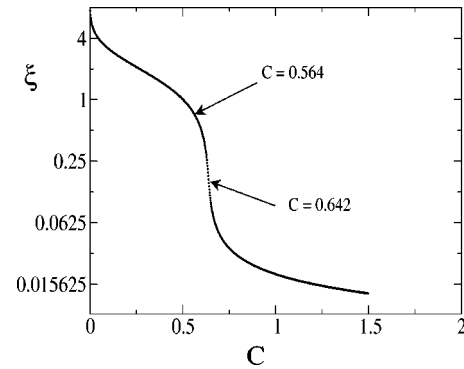
FIG. 2. Inverse of the decay length (in logarithmic scale) as a function of the coupling parameter C , for a fixed value \omega=3\omega_b . We mark two values of C , 0.564, and 0.642, which correspond to two rather different values of \xi , also used in Fig. 3. The rest of the parameters are \omega_b=0.2\pi , \alpha=0.02 , and F_{ac}=0.02 .
