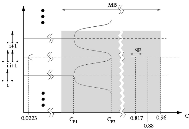
FIG. 8. Scheme showing all bifurcations found in our model up to values of C \approx 1 . The most relevant ones are probably the pitchforks that exchange stability between the one-site and the two-site breather ( C_{p1} , C_{p2} ). At C=0.817 the two-site breather has a subcritical Hopf bifurcation, connecting it to a quasiperiodic breather. At C=0.88 this quasiperiodic solution disappears as it turns into a slow moving breather. The gray-shaded areas between C=0.51 and C=0.96 are those where moving breathers, either fast or slow, can be found.
