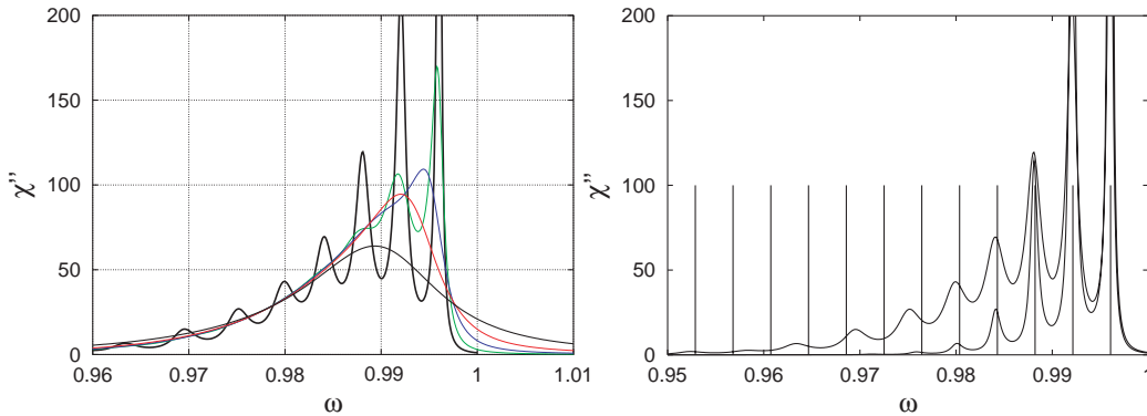
Fig. 3 – Imaginary part of the dynamical susceptibility. Left panel: T = 0.05 and \bar{K} = 200 with \gamma = 0.01, 0.003, 0.001, 0.0003, 0.0001 (bottom to top). Right panel: \gamma = 0.0001 with T = 0.05 and T = 0.025 (lower curve). Vertical lines: transition frequencies of the associated anharmonic oscillator.
