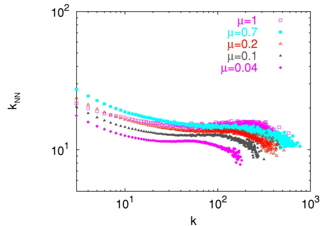
FIG. 5. (Color online) Average nearest neighbor connectivity k_{NN} against k for several values of \mu . Results are averaged over 100 network realizations for each \mu value. Other parameters are as in Fig. 1.
