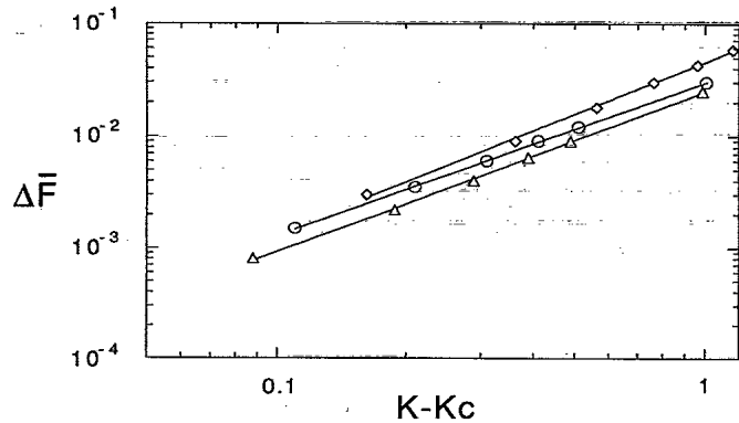
FIG. 4. Log-log plot of the fit by Eq. (11) for the velocities corresponding to ( \Delta ) (r,m,s)=(-1,1,1) , K_c=1.5 , and \xi=1.6 ; ( \circ ) (r,m,s)=(2,-1,1) , K_c=1.9 , and \xi=1.53 ; and ( \diamond ) (r,m,s)=(0,0,1) , K_c=2.4 , and \xi=1.6 .
