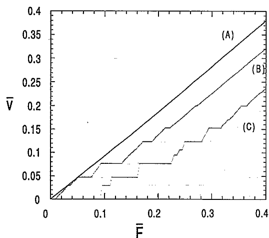
FIG. 2. Response function \bar{v}(\bar{F}) , for F_{ac}=0.2 and v=0.2 . Curve a , K=1.4 [just below the lowest value of K_c(\bar{v}) ]; curve b , K=2.8 ; curve c , K=4 .
