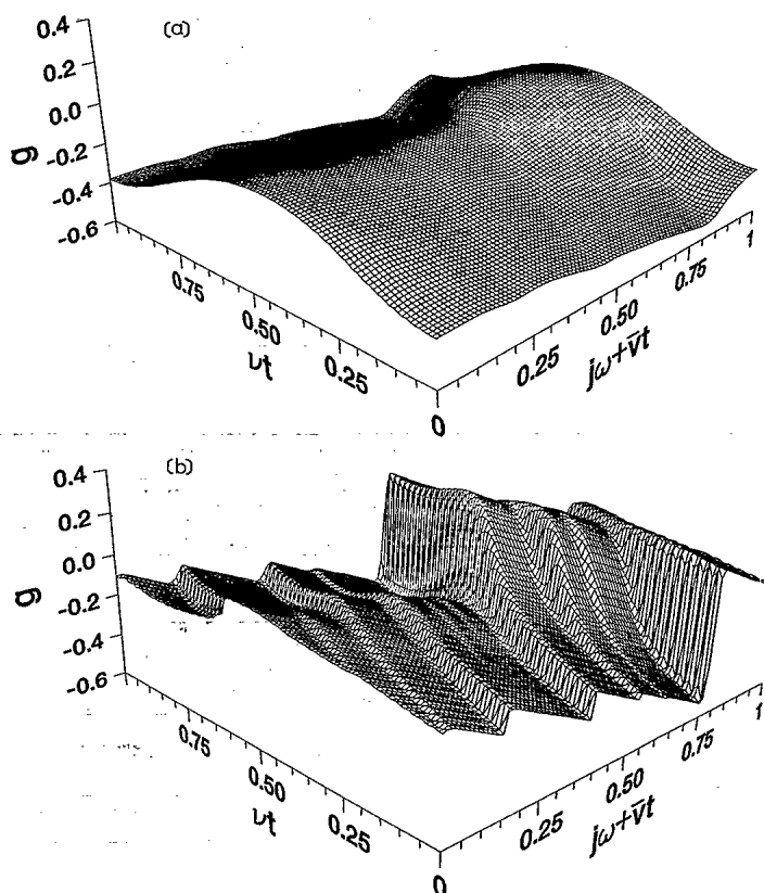
FIG. 3. Two-dimensional hull function g(x,y) describing the motion of the incommensurate structure [see Eq. (9)] for the velocity (10) with r=-1 , m=1 , and s=1 . (a) K=1.4 ; (b) K=4 .
