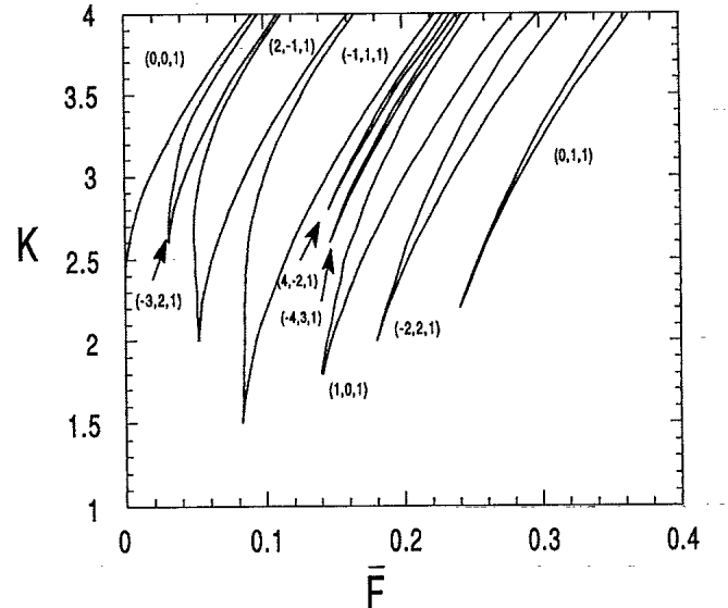
FIG. 1. Phase diagram of the different steady states in the (K, \bar{F}) plane, for F_{ac}=0.2 and \nu=0.2 . The triplets (r, m, s) stand for the integer values in Eq. (10) characterizing the resonant velocity value at which the locking occurs. For the sake of clarity, only tongues corresponding to a few resonant velocities are shown.
