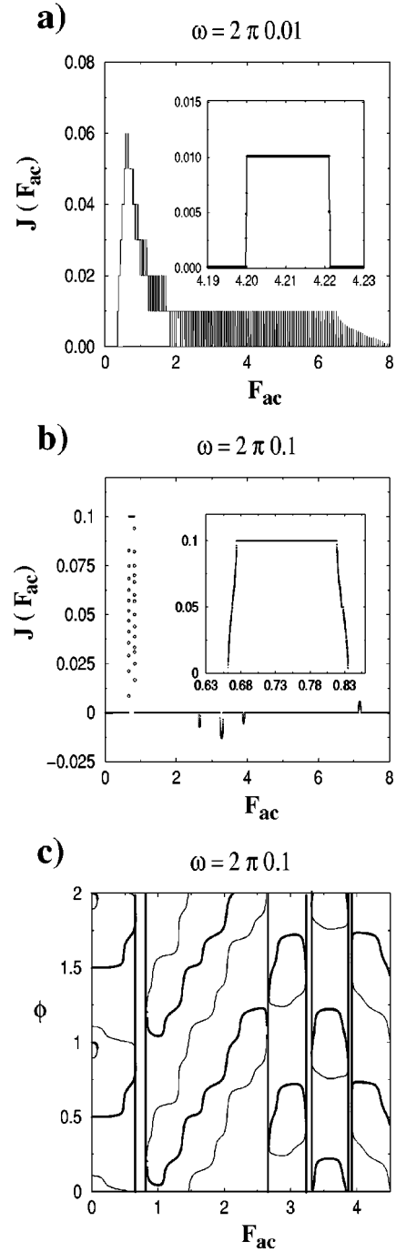
FIG. 1. (a) and (b) Flow as a function of the amplitude of the external force F_{ac} at two different frequency values. (c) Bifurcation diagram using the mean value over a period of u^{tr} \phi = \langle u^{tr} \rangle_T as relevant magnitude for \omega = 2\pi \times 0.1 . Intervals between vertical lines correspond to mobility bands in F_{ac} .
